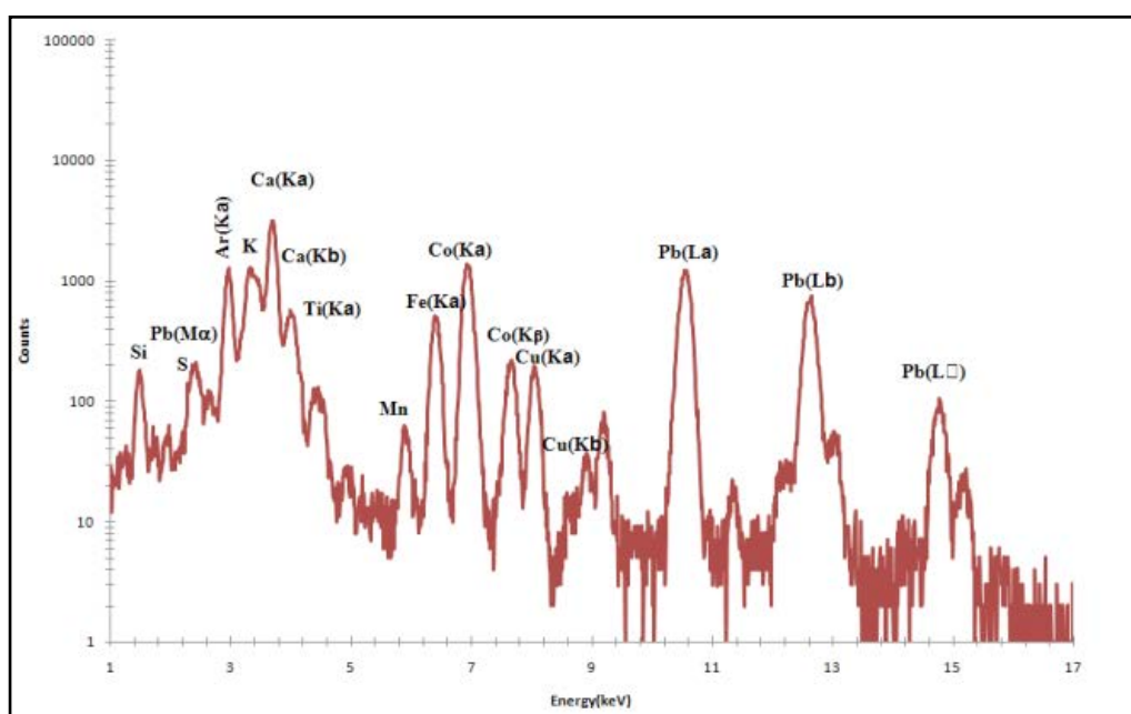
Fig. 15. The PIXE spectrum obtained from the blue pigment of the Zarrinfam tile (Ghadiri, 2013: 24).
